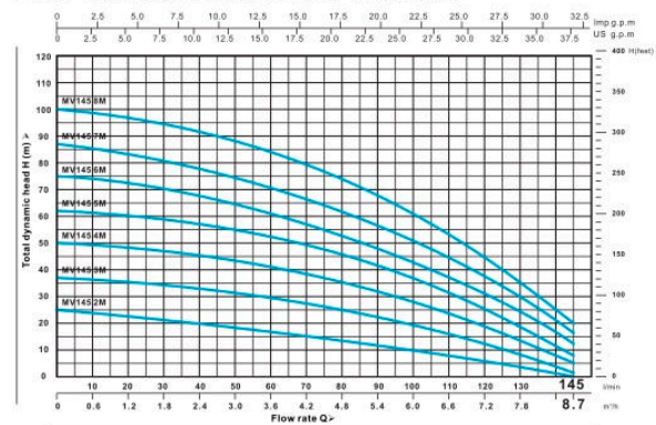
PERFORMANCE DATA AT n= 2850 min -1
